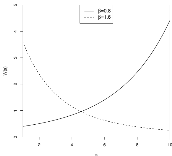
Figure 9.2: Wald Statistic as a Function of s
