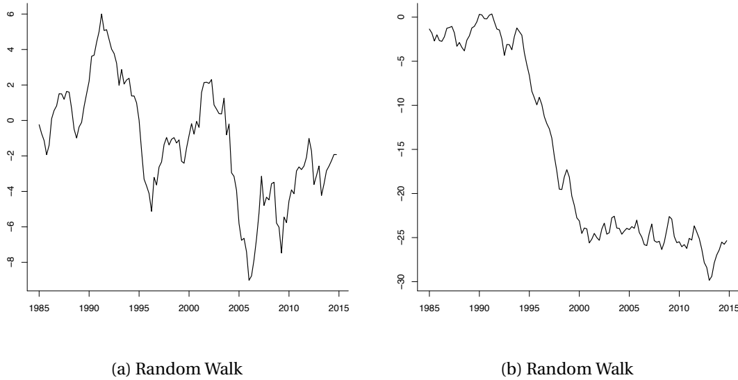
Figure 14.7: Random Walk Processes
