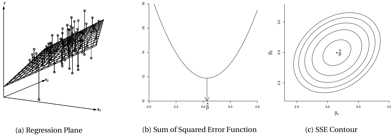
Figure 3.2: Regression with Two Variables
