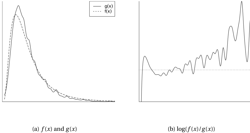
Figure 23.1: Kullback-Leibler Distance Measure
