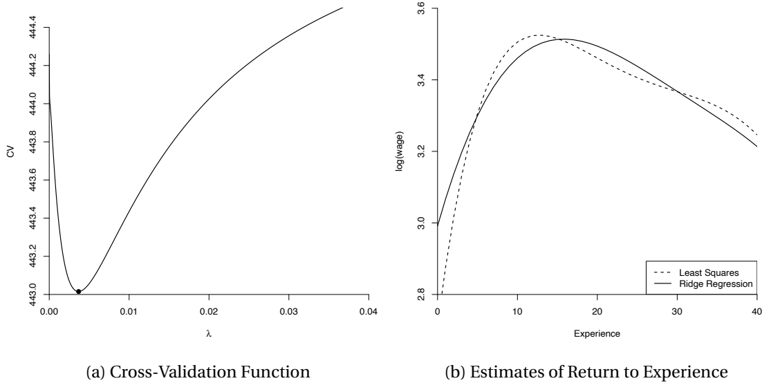
Figure 23.8: Least Squares and Ridge Regression Estimates of the Return to Experience
