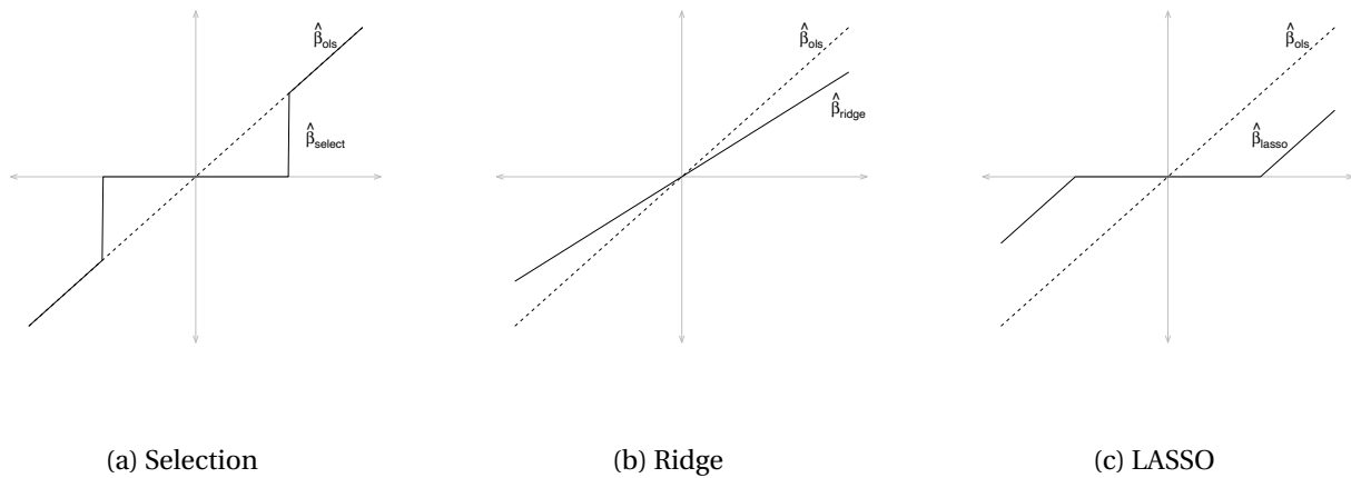
Figure 23.10: Transformations of least squares coefficients by Selection, Ridge, and LASSO estimators
