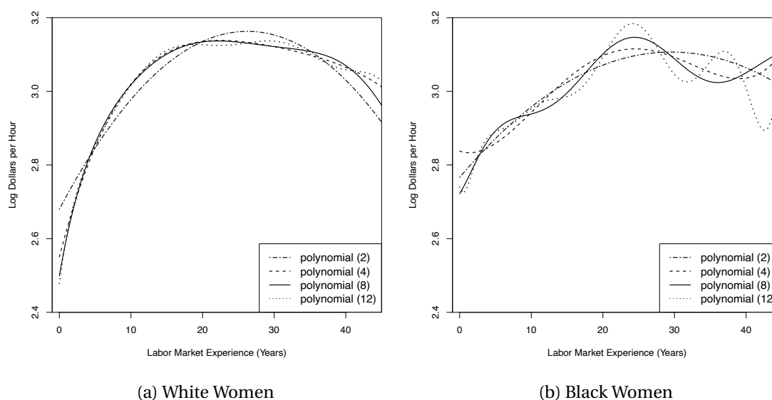
Figure 20.1: Polynomial Estimates of Experience Profile, College-Educated Women
