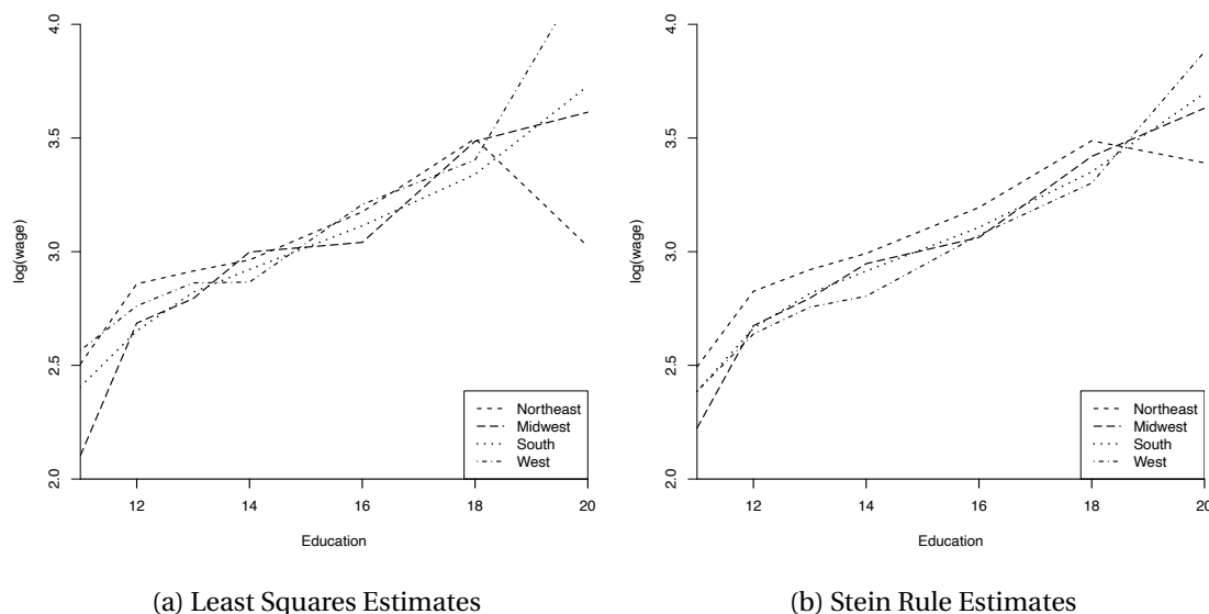
Figure 23.4: Stein Rule Estimation of Education Profiles Across Regions
