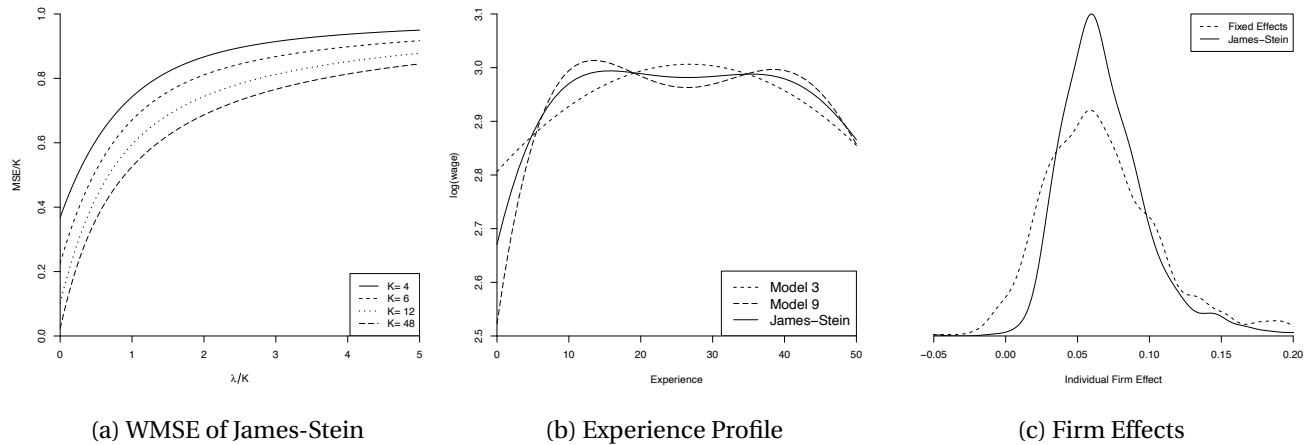
Figure 23.3: James-Stein Estimator
