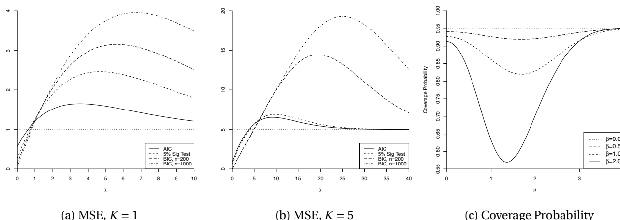
Figure 23.2: MSE and Coverage of Post-Model-Selection Estimators
