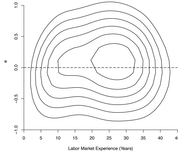
Figure 2.5: Joint Density of Error e and experience for White Men with High School Education
