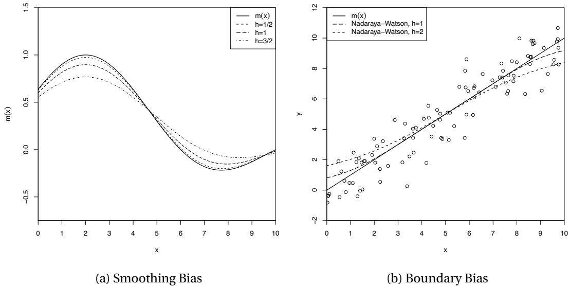
Figure 19.2: Asymptotic Bias
