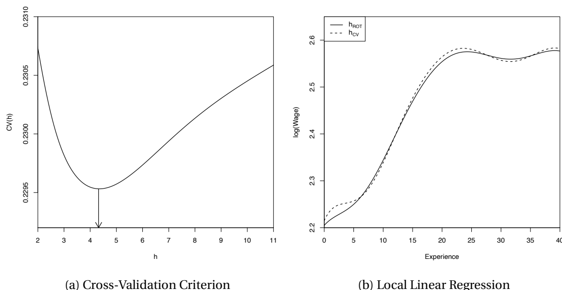
Figure 19.4: log(wage) regression on experience
