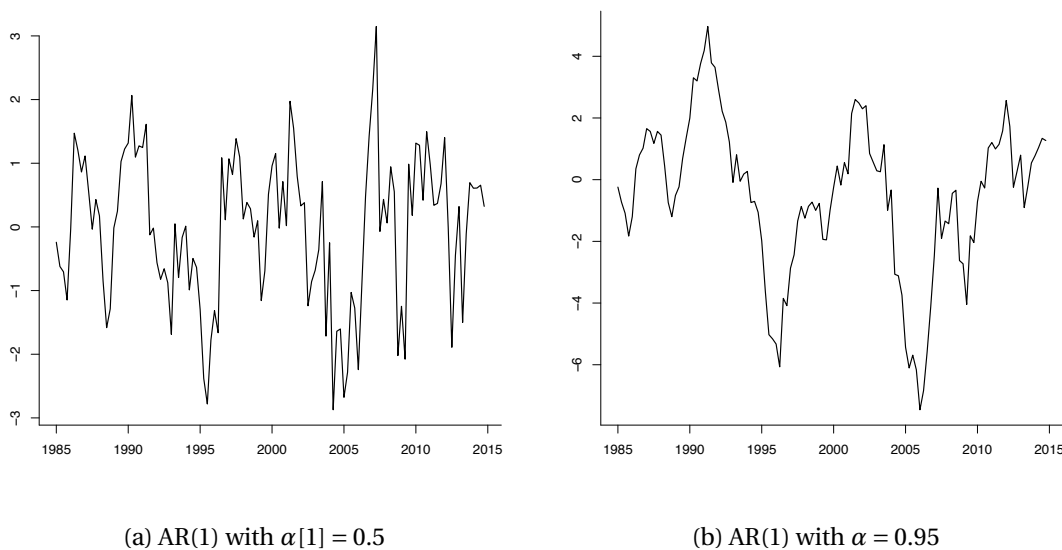
Figure 14.6: AR(1) Processes
